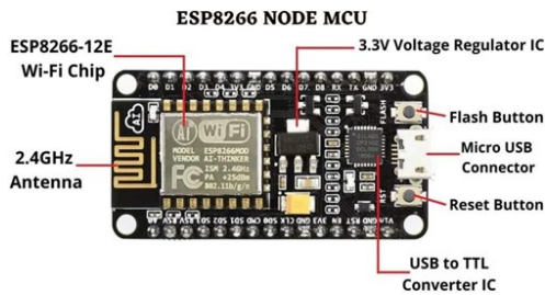
Figure 5: NodeMCU Parts
